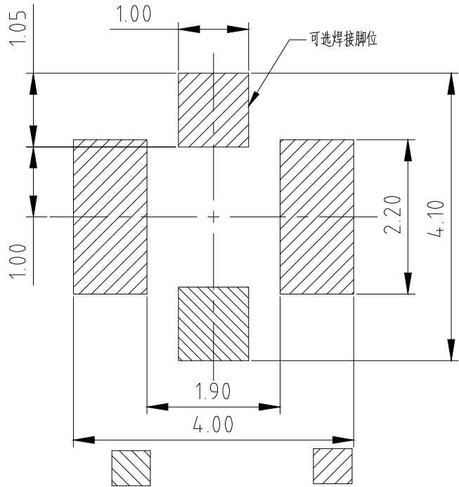
SIGNAL CONTACT GROUND CONTACT P.C.B DIMENSION (TOP VIEW) (TOLERRANCE ±0.05)
