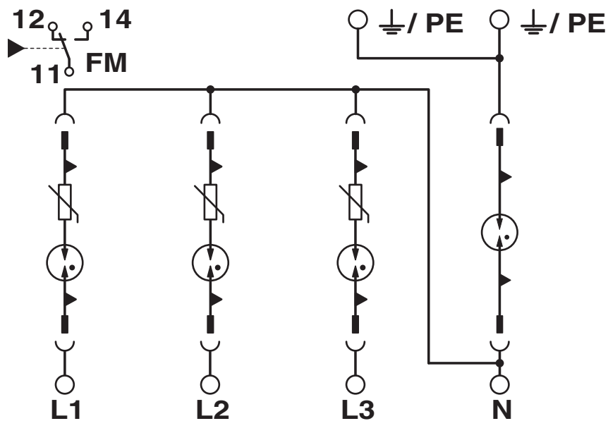
Circuit diagram
