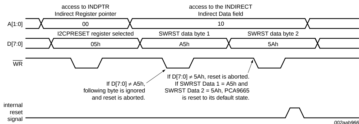
Fig 17. Parallel Software Reset sequence
