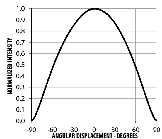
Figure 12 Radiation Pattern
