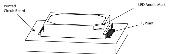
Figure 18 LED Solder Point
