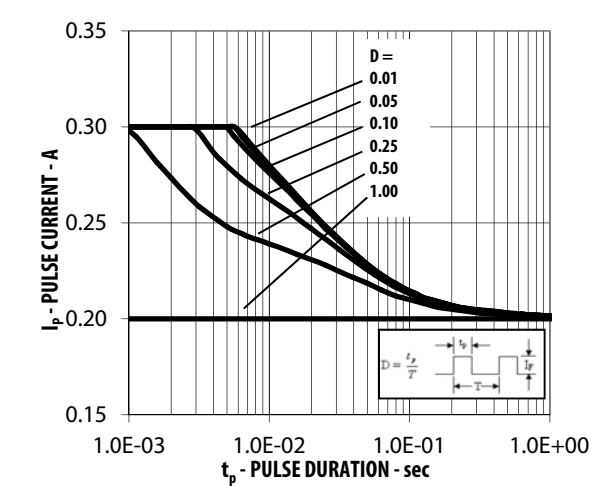
Figure 11 Pulse Handling Capability at T S ≤ 100 °C
