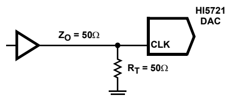
FIGURE 18. AC TERMINATION OF THE HI5721 CLOCK LINE
