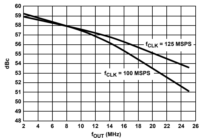
FIGURE 9. SPURIOUS FREE DYNAMIC RANGE (TO NYQUIST) vs OUTPUT FREQUENCY
