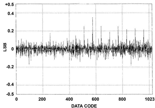
FIGURE 5. DIFFERENTIAL NON-LINEARITY
