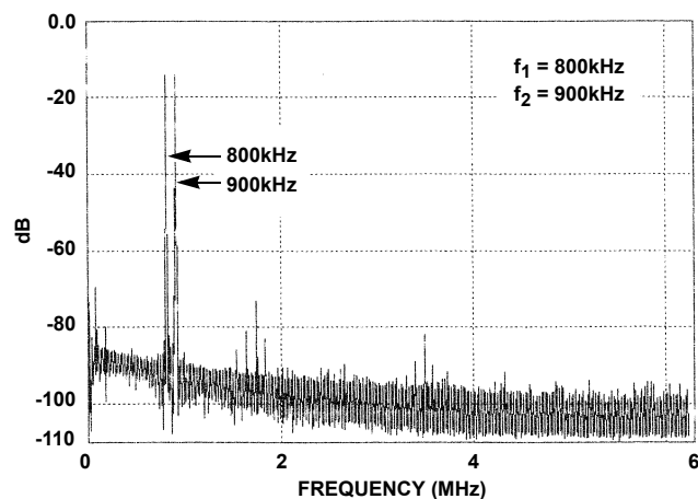
FIGURE 8. INTERMODULATION DISTORTION
