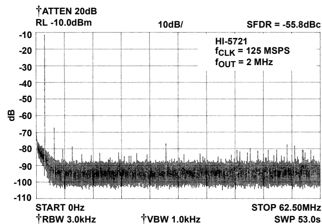
FIGURE 7. SPURIOUS FREE DYNAMIC RANGE TO NYQUIST 2MHz FUNDAMENTAL
