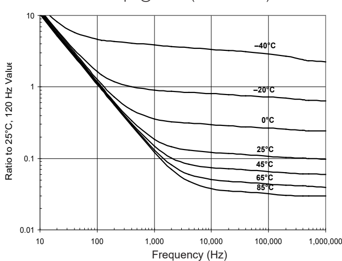
Impedance vs. Temperature and Frequency 100 \mu F @ 16 Vdc (10 X 10.2 mm)
