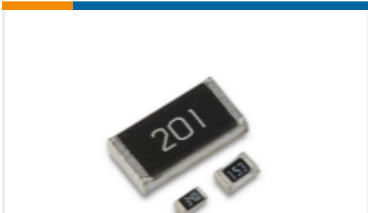
TE Part #3-2176325-8 CRGP 0402 12K 1%
