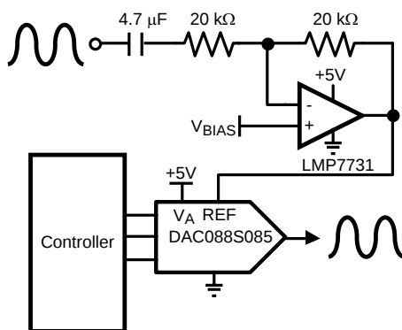
Figure 40. Programmable Attenuator
