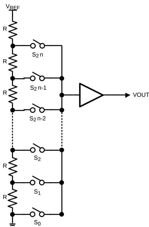
Figure 27. DAC Resistor String
