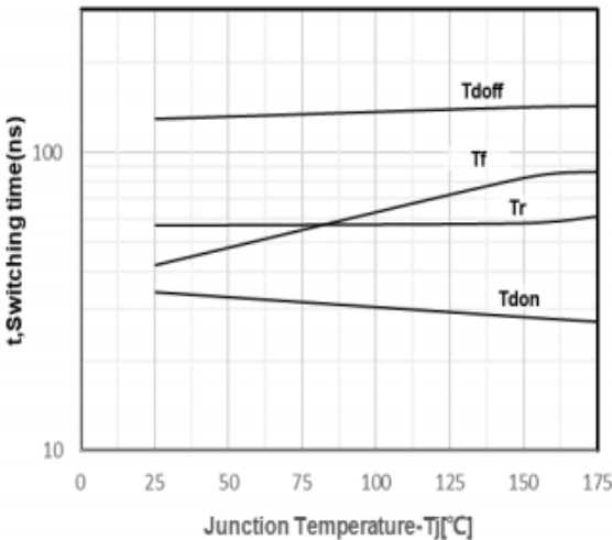
Typ. Switching times as a function of junction temperature (inductive load, V_{CE}=400\text{V} , V_{GE}=0/15\text{V} , R_G=10\Omega )
