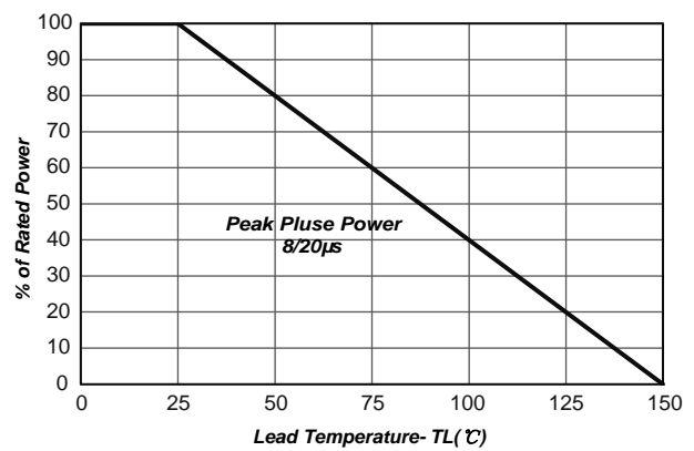
Fig2. Power Derating
