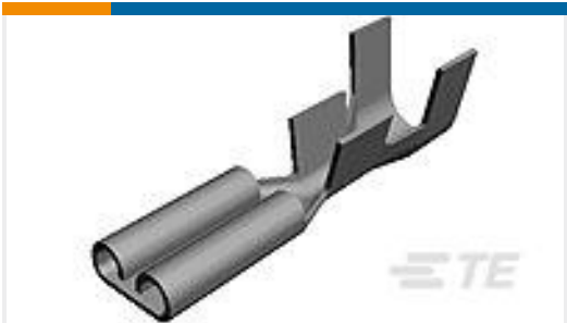
TE Part #140825-2 110 FASTON,REC.,22-18 AWG,PTBR
