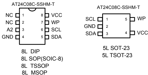
Figure 1: Package types
