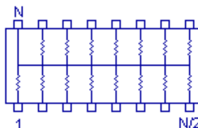
Bussed CTS Schematic 1
