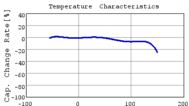
Temperature [degC] RHEL82A103K0K1H03B C-Temp. capchange, DCOV,
