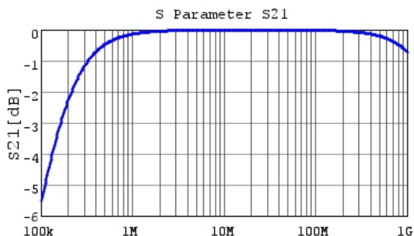
Frequency [Hz] RHEL82A103K0K1H03B S21 DCOV, 25degC
