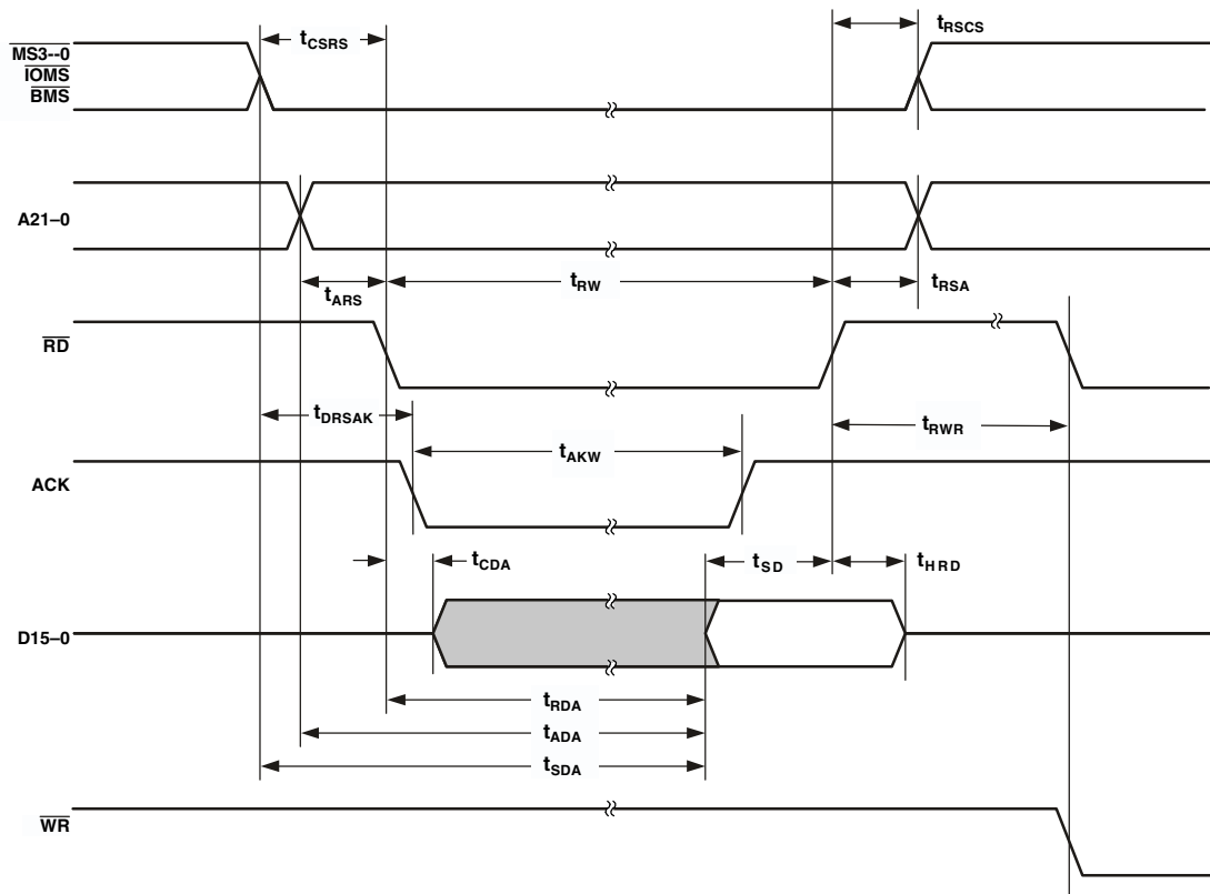
Figure 10. External Port Read Cycle Timing
