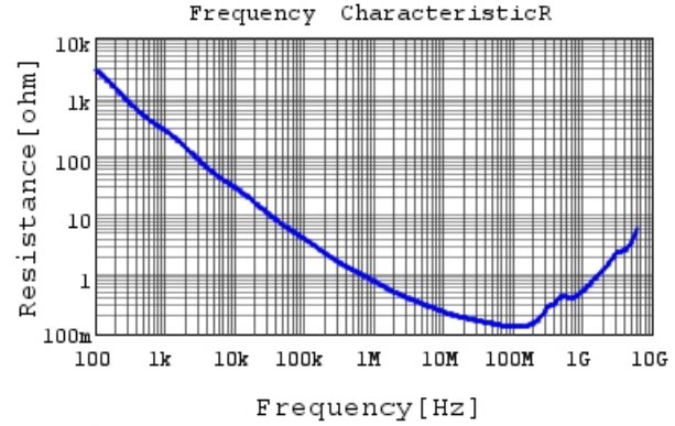
GCD188R71H272MA01 R DCOV, 25degC
