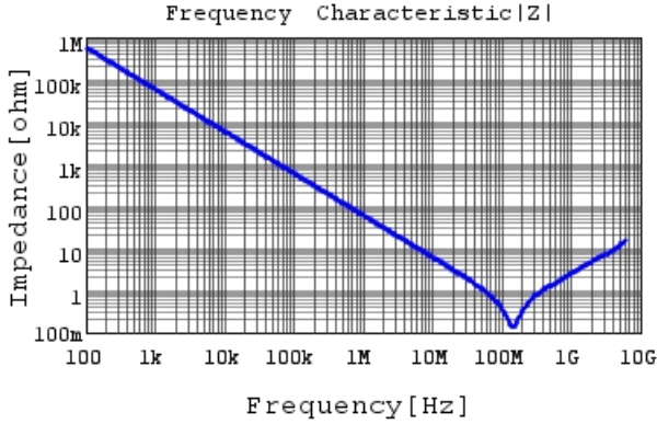
GCD188R71H272MA01 |Z| DCOV, 25degC
