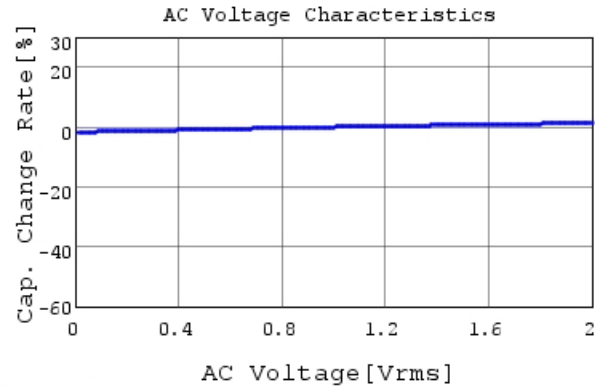
GCD188R71H272MA01 C-AC Voltage capchange, Dc
