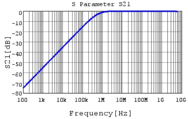
GCD188R71H272MA01 S21 DC0V, 25degC
