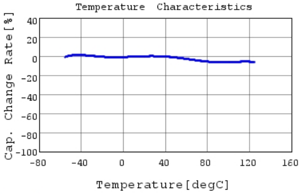
GCD188R71H272MA01 C-Temp. capchange, DC0.0V,
