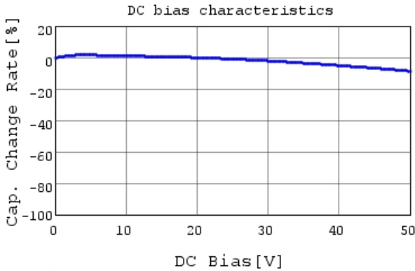
GCD188R71H272MA01 C-DC bias capchange, 25.0c
