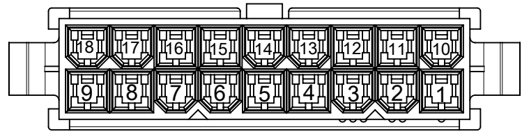
18 CKTS.
