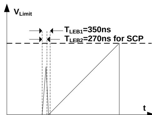
Figure 11: Leading-Edge Blanking
