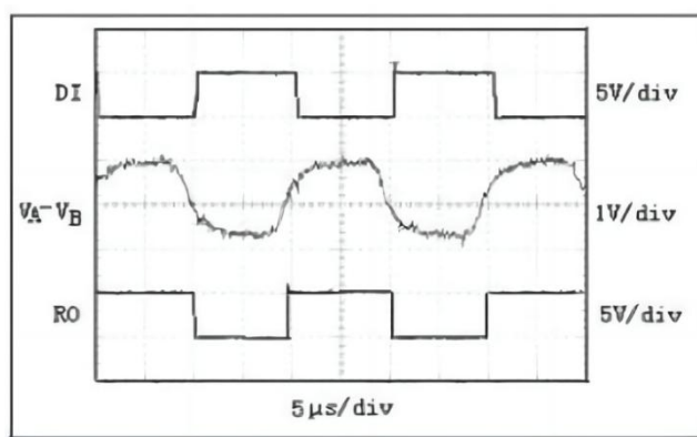
Figure 10: Driving 4000 ft cable at 50kHz MAX490 system differential voltage linear transponder
