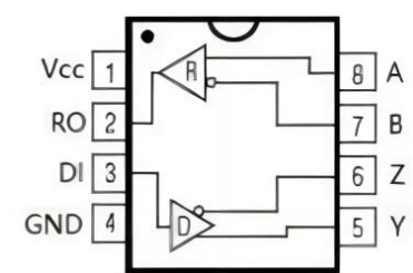
DIP/SOP
