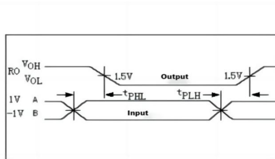
Figure 7: Receiver propagation delay
