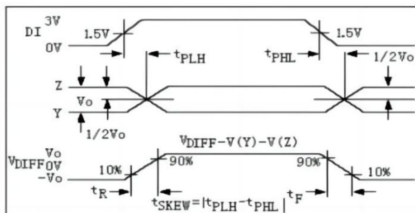
Figure 6: Driver propagation delay
