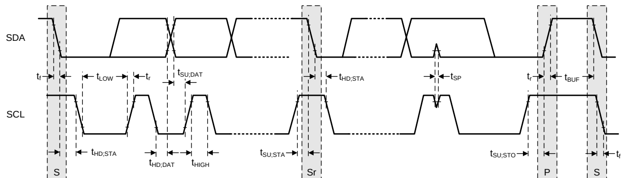
Figure 5-34. I²C Protocol and Transmission Timing; I²C Data Transmission Timing
