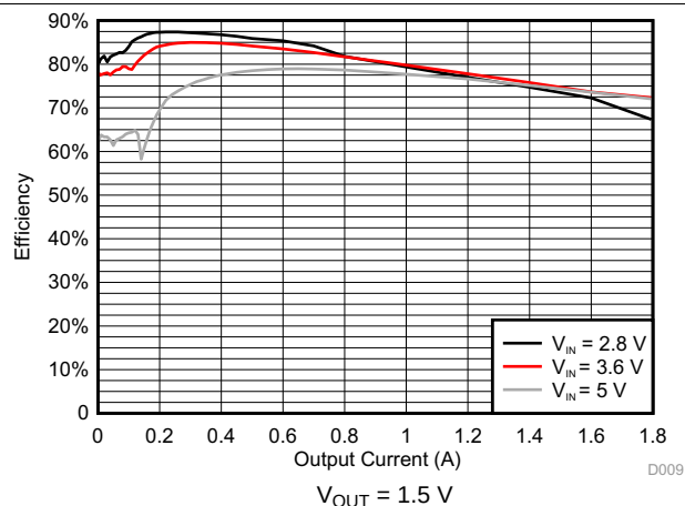
Figure 6-6. DCDC3 Efficiency
