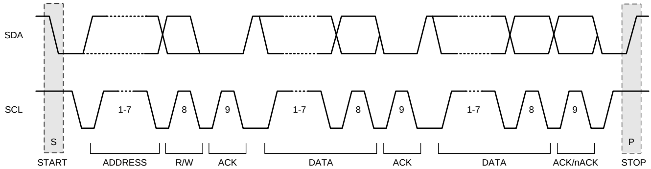
Figure 5-33. I²C Protocol and Transmission Timing; I²C Start/Stop/Acknowledge Protocol
