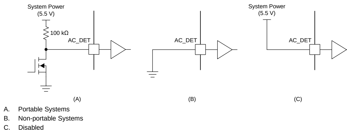
Figure 5-28. AC_DET Pin Configurations
