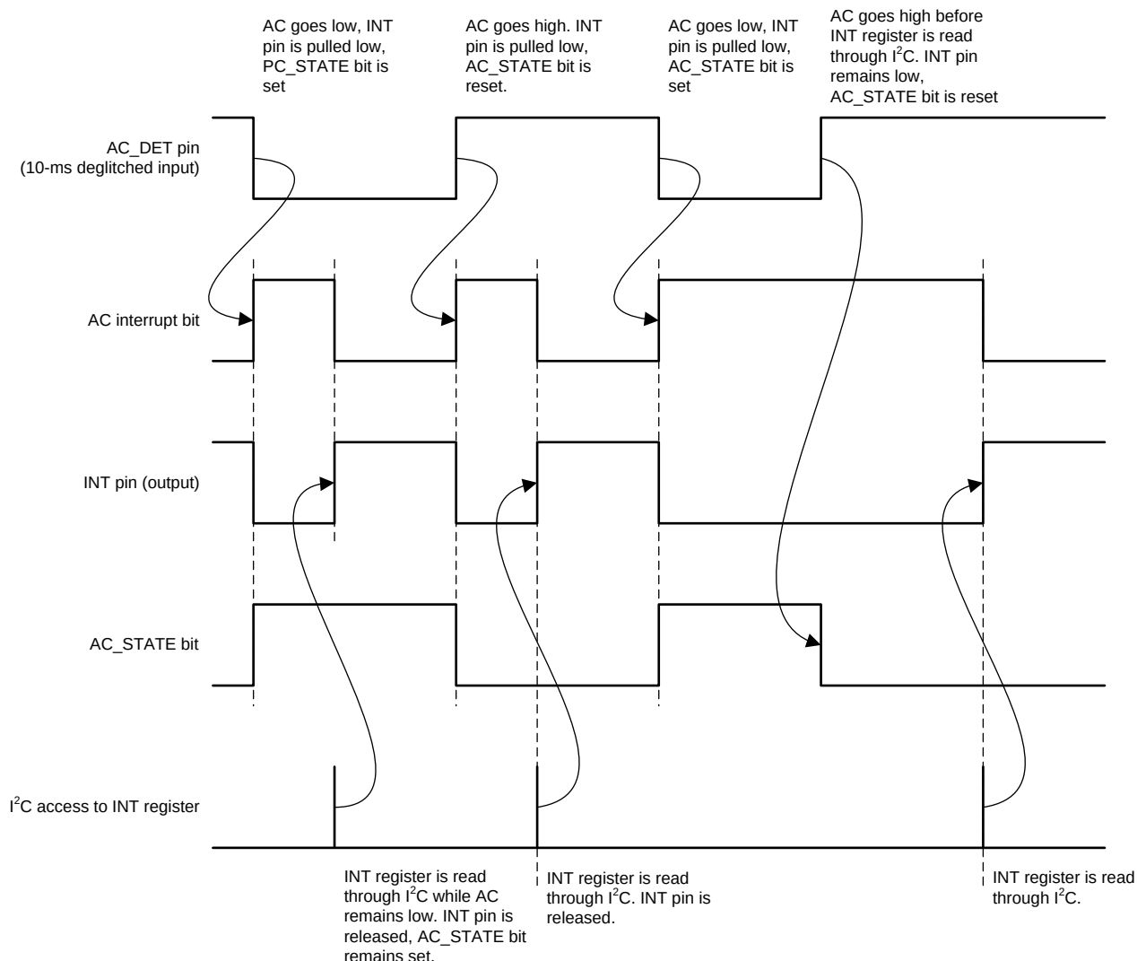
Figure 5-30. AC_STATE Pin
