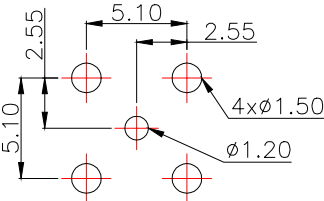
PCB.WELDING DRAWING (TOLERANCE:±0.05)
