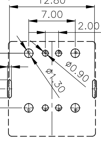
P. C. B LAYOUT
