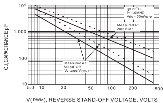
Fig.4 TYPICAL CAPACITANCE
