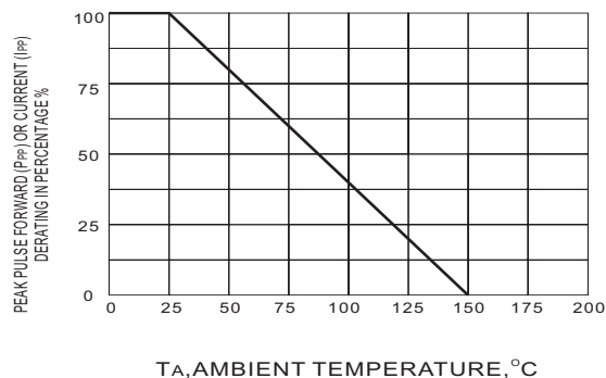
Fig.2 DERATING CURVE
