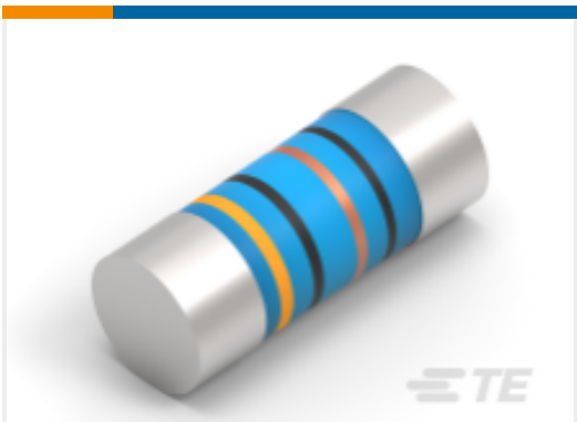
TE Part #3-2176316-2 MELF SMA_A 39K 0.1% 15PPM 0207 1W
