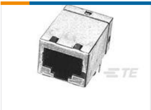
TE Part #1734795-1 RJ45,8P8C,SHD,W/O LED,DIP 6u"
