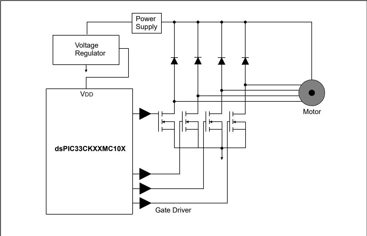
FIGURE 2-5: STEPPER MOTOR
