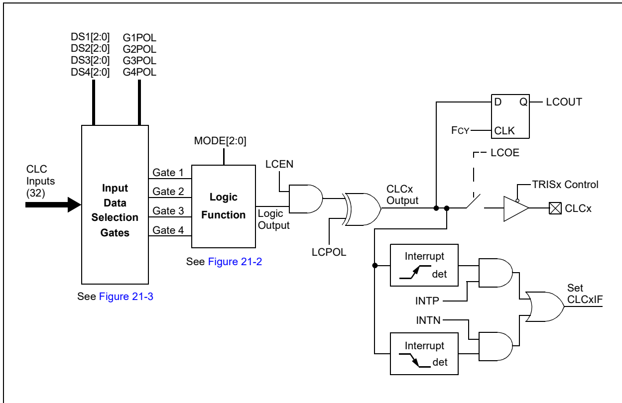
FIGURE 21-1: CLCx MODULE
