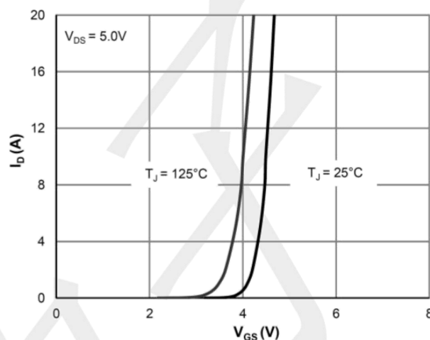
Transfer Characteristics
