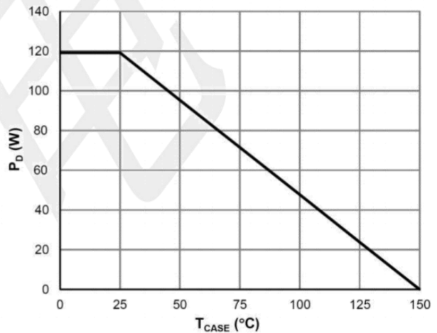
Power De-rating
