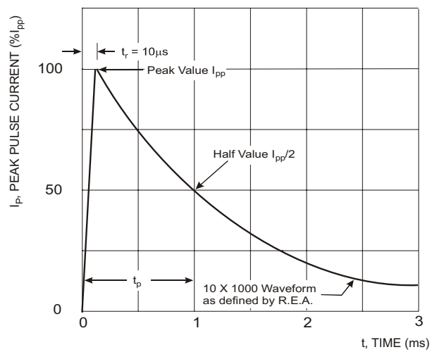
Fig. 4 Pulse Waveform
