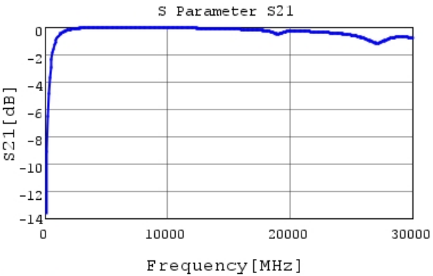
GJM0335G2A3R4BB01 S21 DCOV, 25degC
