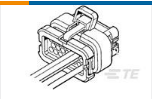
TE Part #770680-2 23POS,AMPSEAL,SOC HSG ASSY,SLD, COD 2
