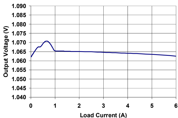
Fig. 20: Load Regulation
