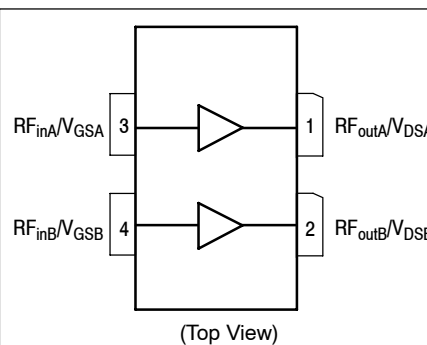
Figure 1. Pin Connections
