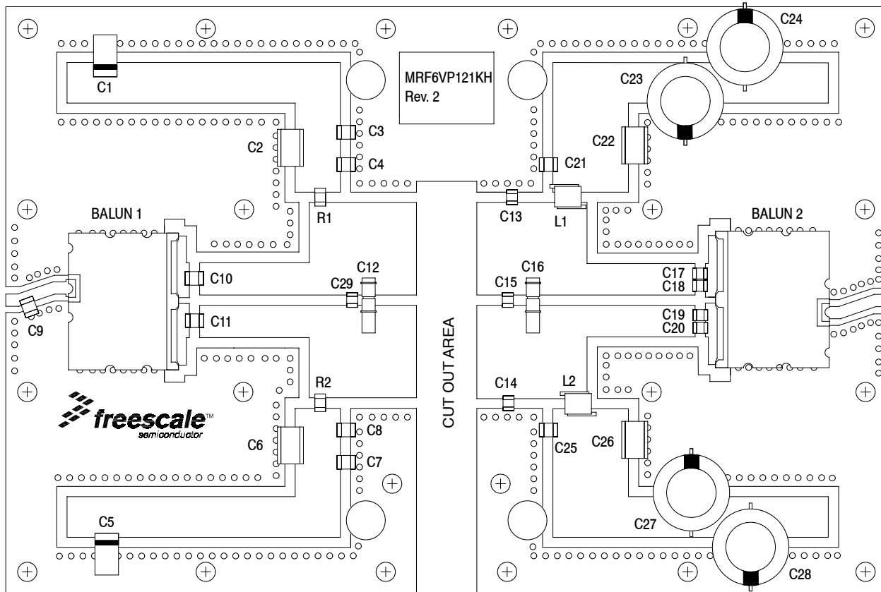
Figure 17. MRF6VP121K6(HSR6) Test Circuit Component Layout — 1090 MHz
