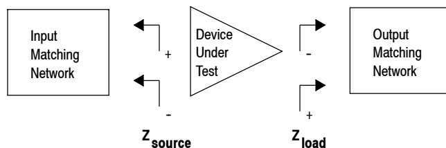
Figure 19. Series Equivalent Source and Load Impedance — 1090 MHz
