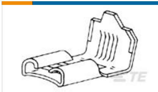
TE Part #62056-6 250 FASTON FLAG REC 18-12 AWG TPBZ
