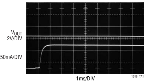
USB SEPIC Start-Up with Output Shorted
