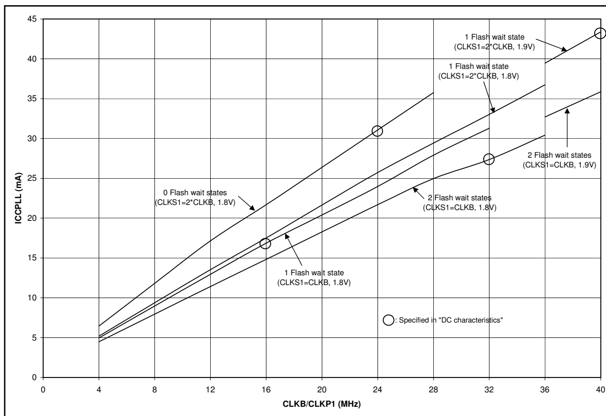
MB96F388/F389 PLL Run mode currents
