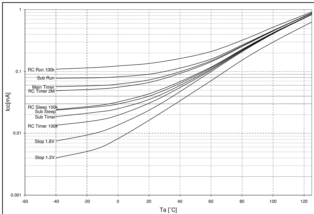
MB96F386/F387 Low power mode currents
