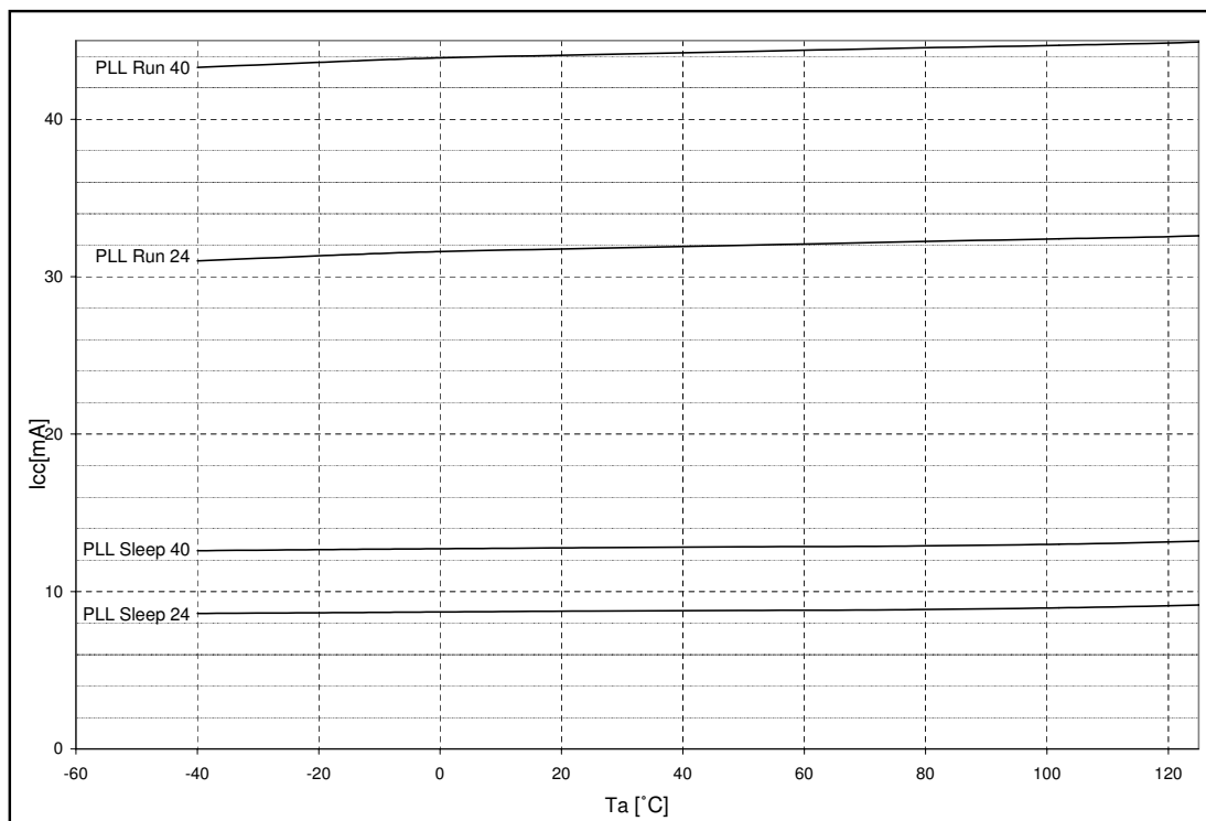
MB96F388/F389 PLL Run and Sleep mode currents
