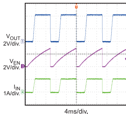
Figure 7: Auto-Retry Waveform
