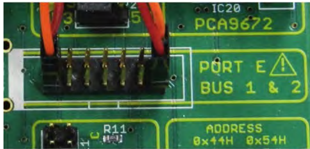
Fig 8. OM13260 Port E jumper
