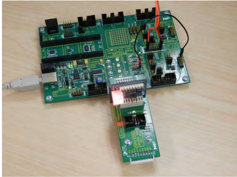
Fig 79. Bridge board (OM13399) used to attach a PCA9632 (OM13269)
