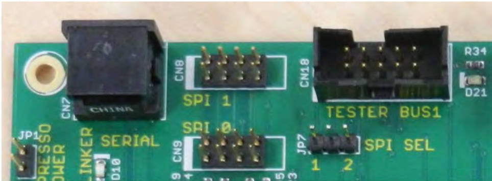
Fig 45. SPI 0 and SPI 1 (Bus2 LPC Xpresso) connectors
