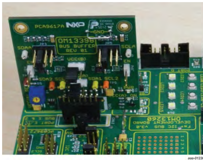
Fig 65. Bus buffer board (OM13398) attached to the Fm+ development board (OM13260)
