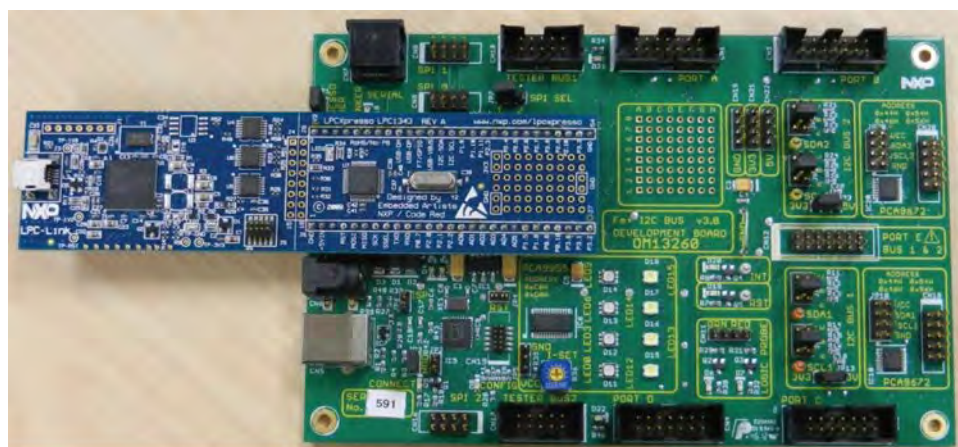
Fig 26. Fm+ development board with LPC Xpresso installed
