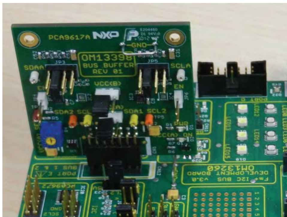
Fig 36. Port E with bus buffer card (OM13398) installed
