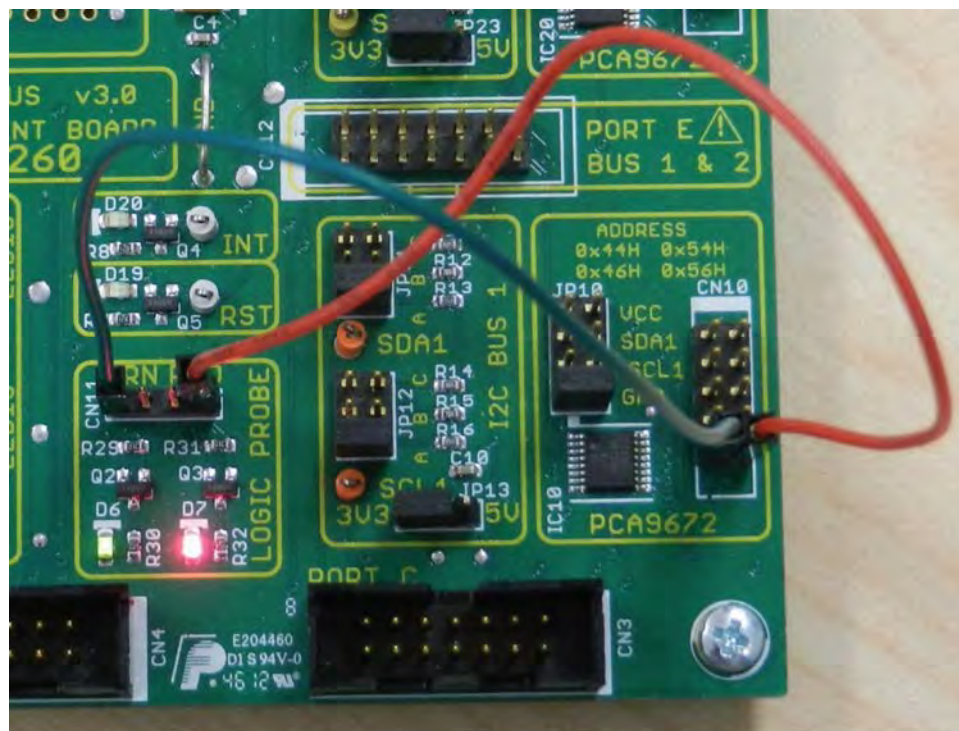
Fig 47. Logic probe section (shown monitoring two GPIO channels from Bus1)
