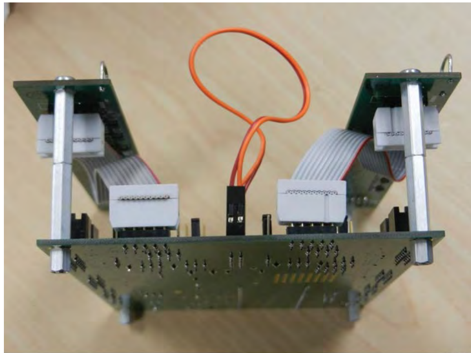
Fig 62. Ribbon cables attached to underside of the GPIO target board (OM13303)
