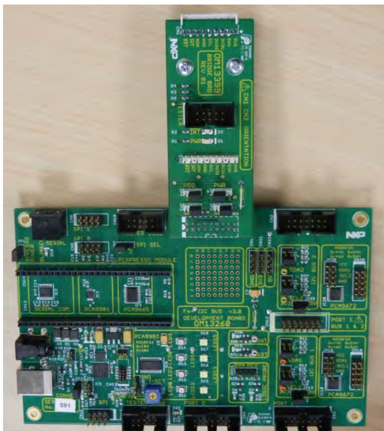
Fig 72. Bridge board (OM13399) attached to the Fm+ development board (OM13260)
