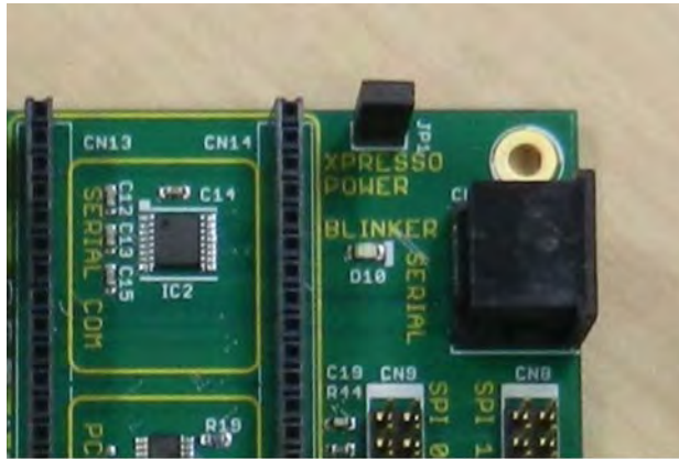
Fig 27. LPC Xpresso power (JP1)
