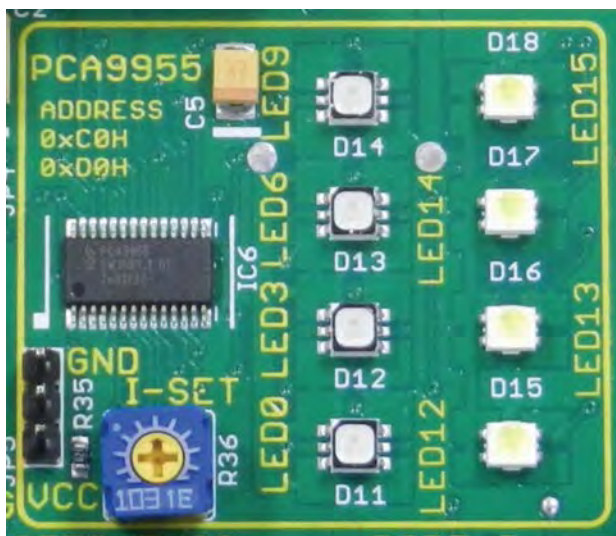
Fig 22. Bus1 LED driver 16-channel section
