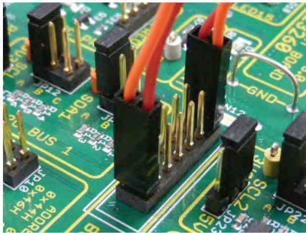
Fig 35. Port E with wire jumper
