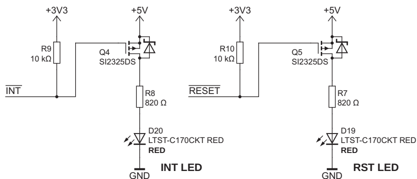
Fig 48. INT and RST indicators circuit
