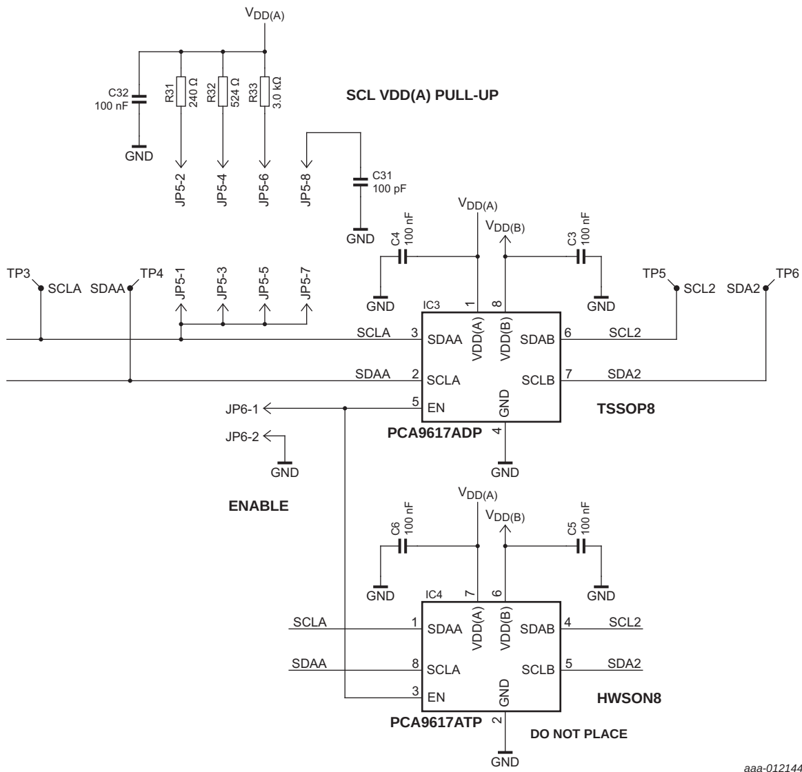
Fig 68. Bus2 bus buffer
