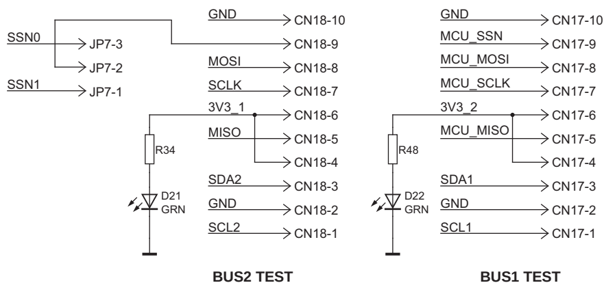
Fig 37. Bus1 and Bus2 tester connectors
