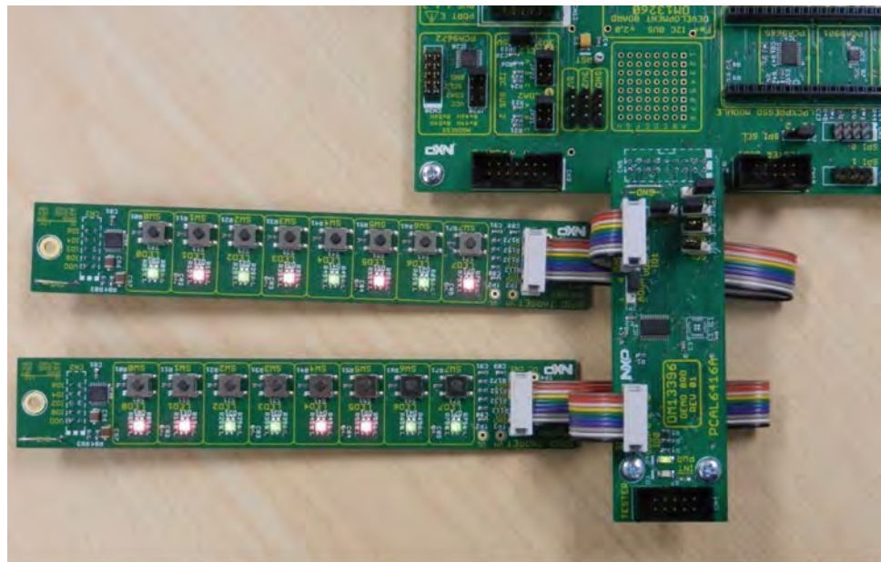
Fig 63. Ribbon cables attached to the topside of the GPIO target board (OM13303)
