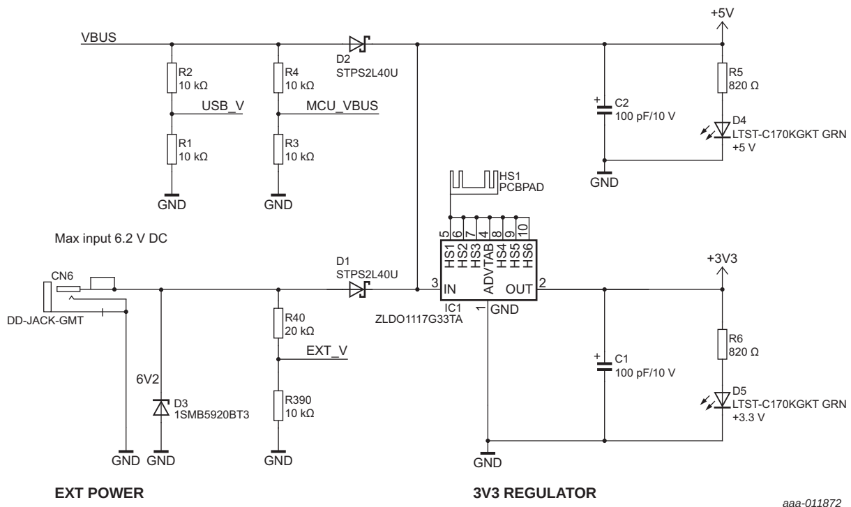
Fig 11. Power supply
