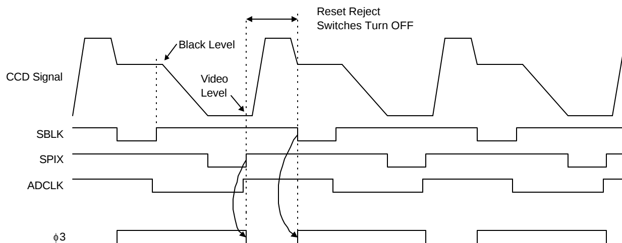
Figure 17. Pixel Rate Clock Timing with RSTreject=1
