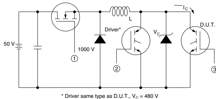
Fig. 14a - Switching Lost Test Circuit
