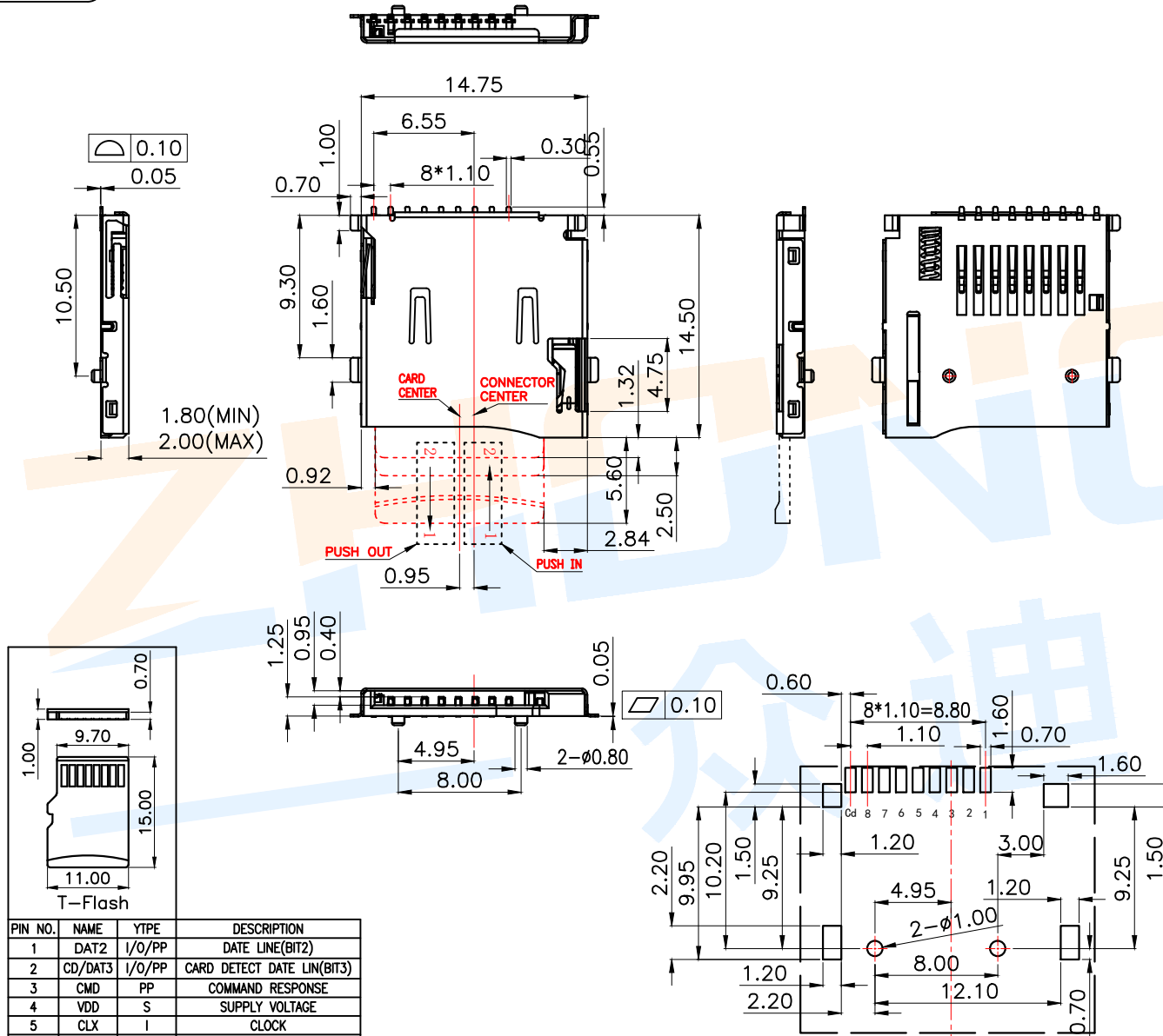
RECOMMENDED P.C.B HOLE LAYOUT COMPONENT SIDE VIEW(TOLERANCE: +/-0.05)
