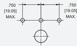
Three Pole*
