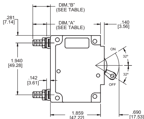
Two Pole
