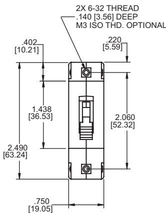
Screw Terminal
