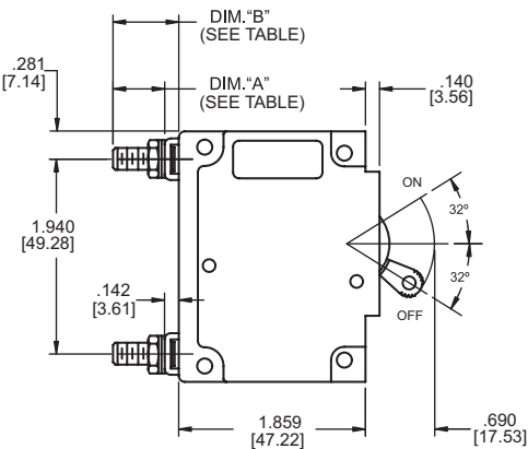
Single Pole
