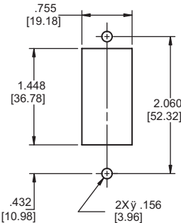
Mounting Detail
