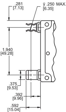
Clip Terminal
