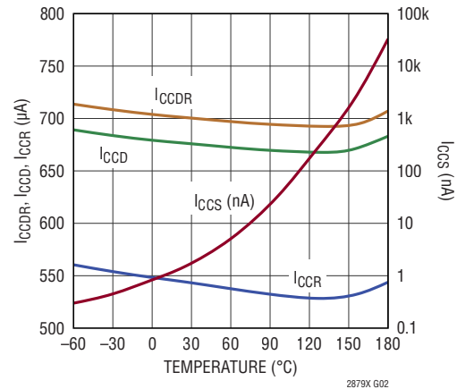
V_{CC} Supply Current vs Temperature for Various Modes, No Load
