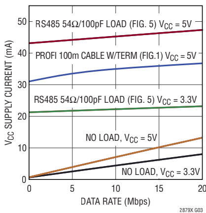
V_{CC} Supply Current vs Data Rate
