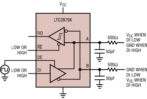
Figure 6. Driver Enable, Disable and Shutdown Timing Measurements
