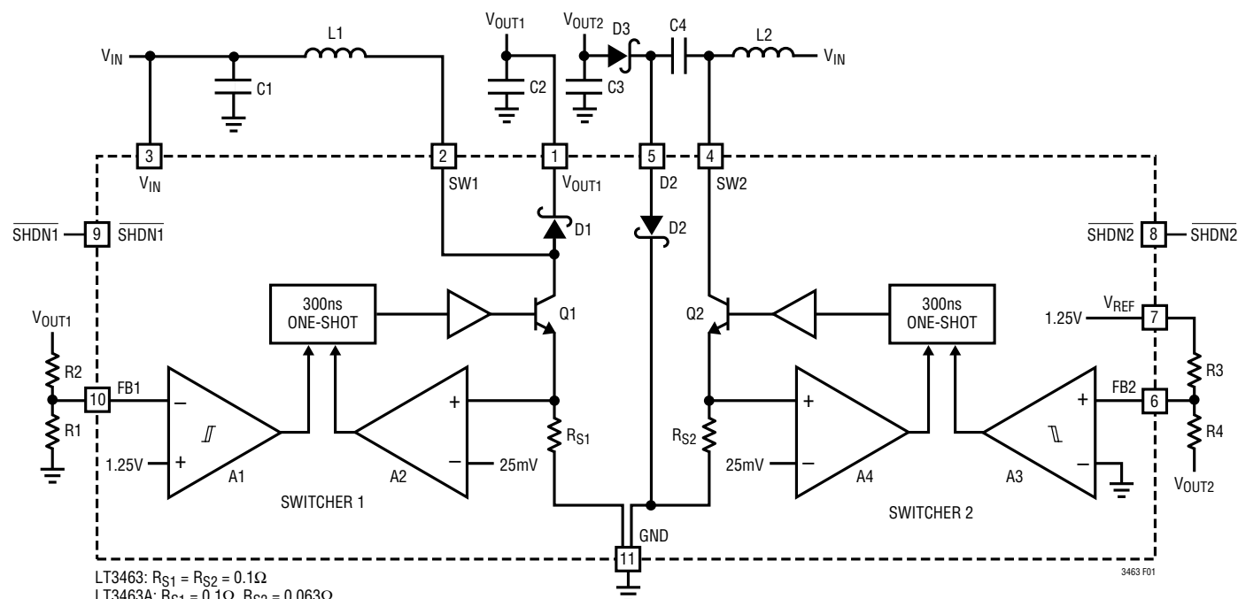
Figure 1. Block Diagram
