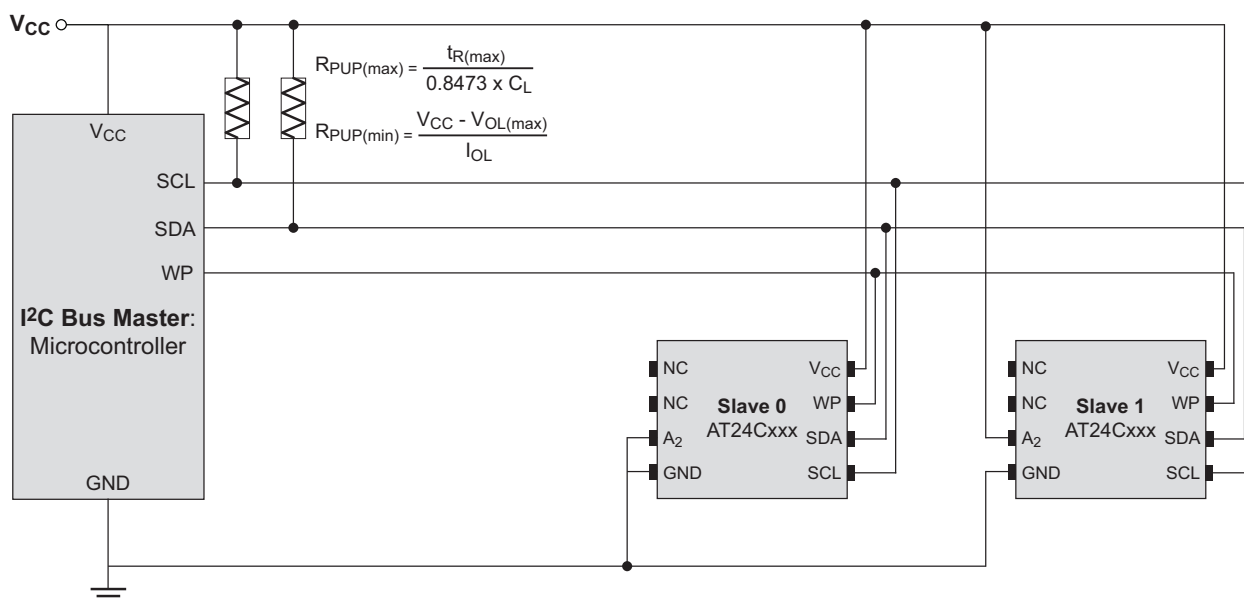
Figure 2-2. System Configuration Using 2-Wire Serial EEPROMs
