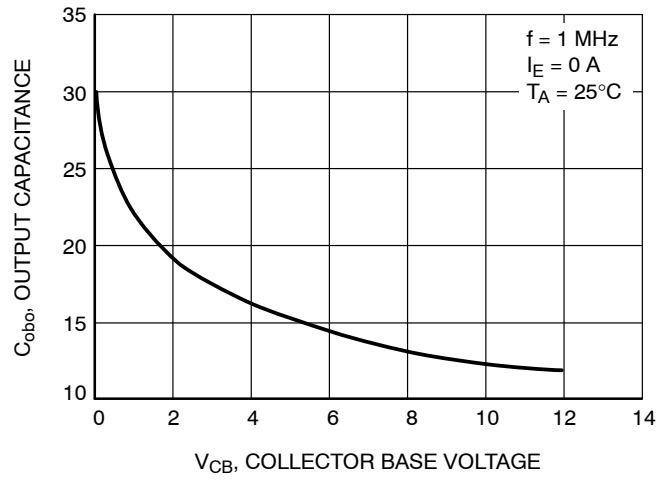
Figure 15. Output Capacitance
