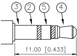
ø2.5 MATING PLUG
