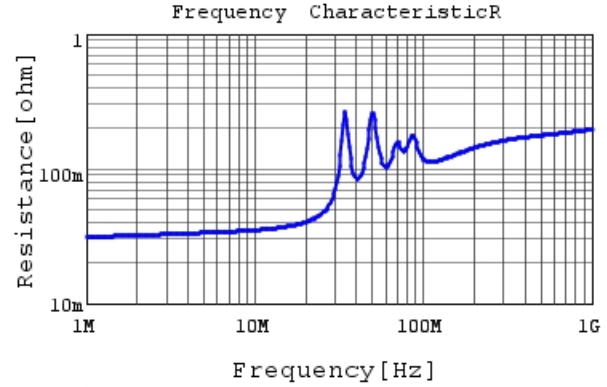
RDE5C1H823J2K1H03B R DC0V, 25degC
