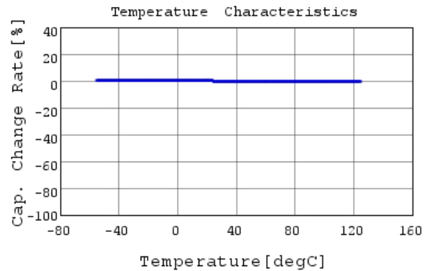
RDE5C1H823J2K1H03B C-Temp. capchange, DC0V,
