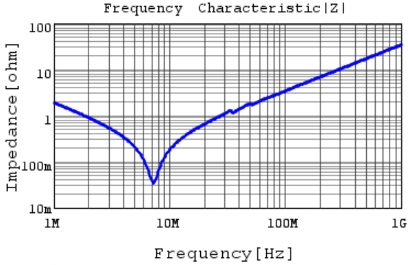
RDE5C1H823J2K1H03B |Z| DC0V, 25degC
