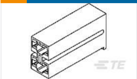
TE Part #172210-7 POSITIVE LOCK 250 HOUSING RECEPTACLE
