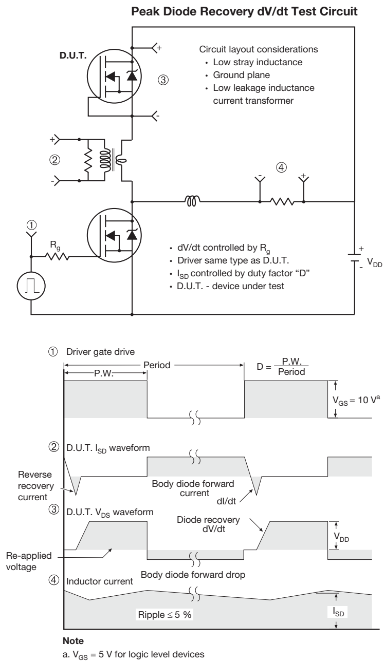
Fig. 18 - For N-Channel
