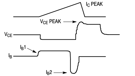
Figure 19. Inductive Switching Measurements
