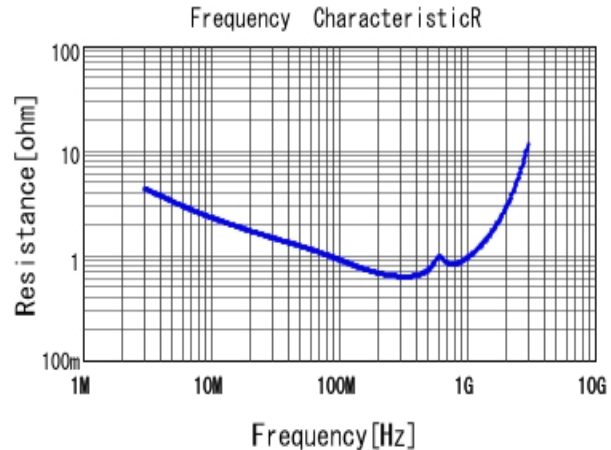
■ GR442QR73D271KW01 R DC0V, 25degC
