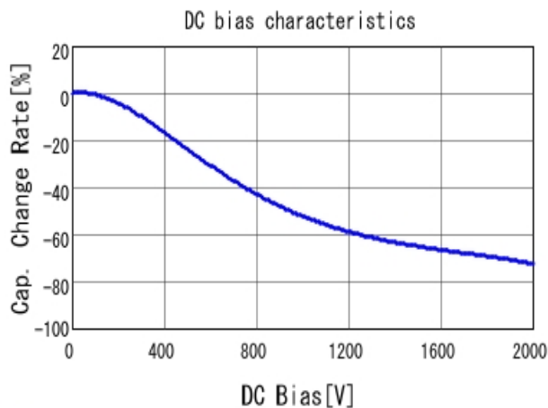
■ GR442QR73D271KW01 C-DC bias capchange, 25.0degC, AC1V
