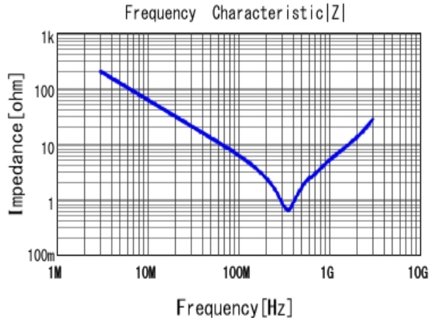
■ GR442QR73D271KW01 |Z| DC0V, 25degC
