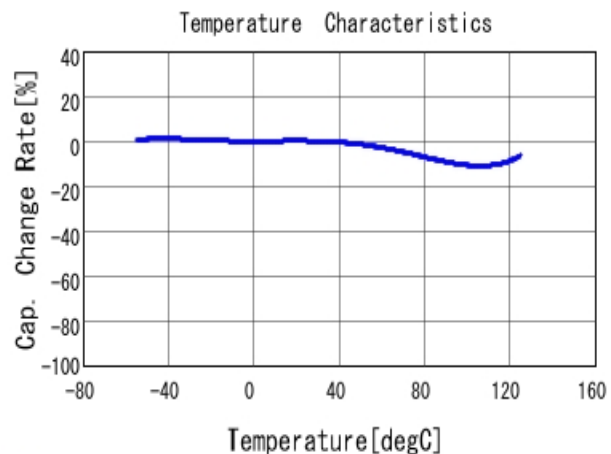
■ GR442QR73D271KW01 C-Temp. capchange, DC0V, AC1Vrms
